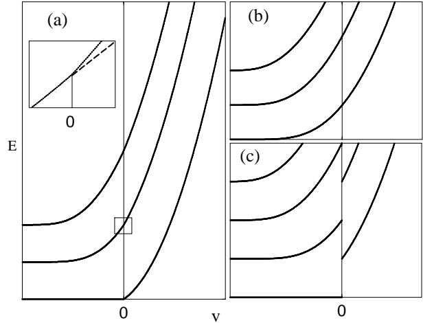
Fig. 1. Spectrum of Landau Hamiltonians: (a) with chiral boundary conditions (inset: enlarged box, showing a cusp between bulk and edge states), (b) with Dirichlet boundary conditions, (c) with APS boundary conditions.
